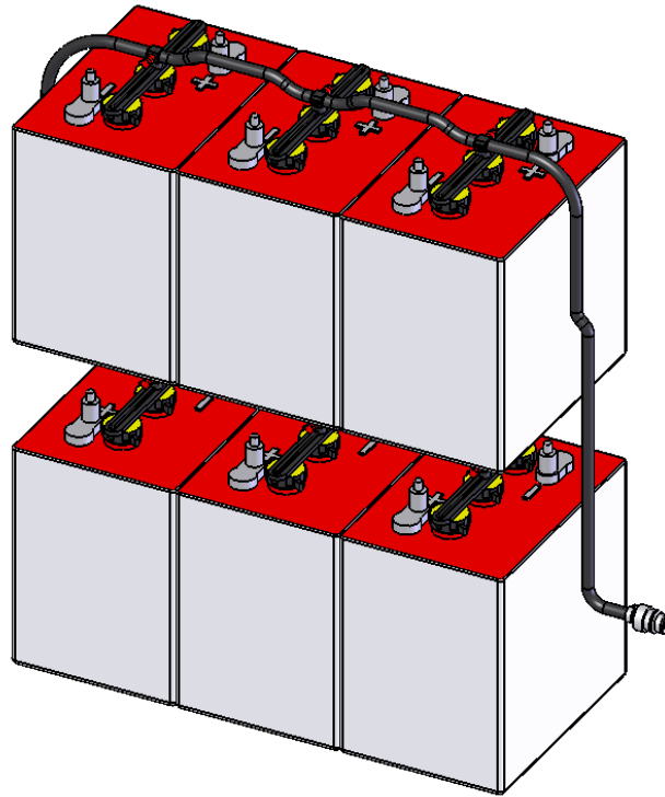
PRO-FILL WATERING SYSTEM - PART # E012613
